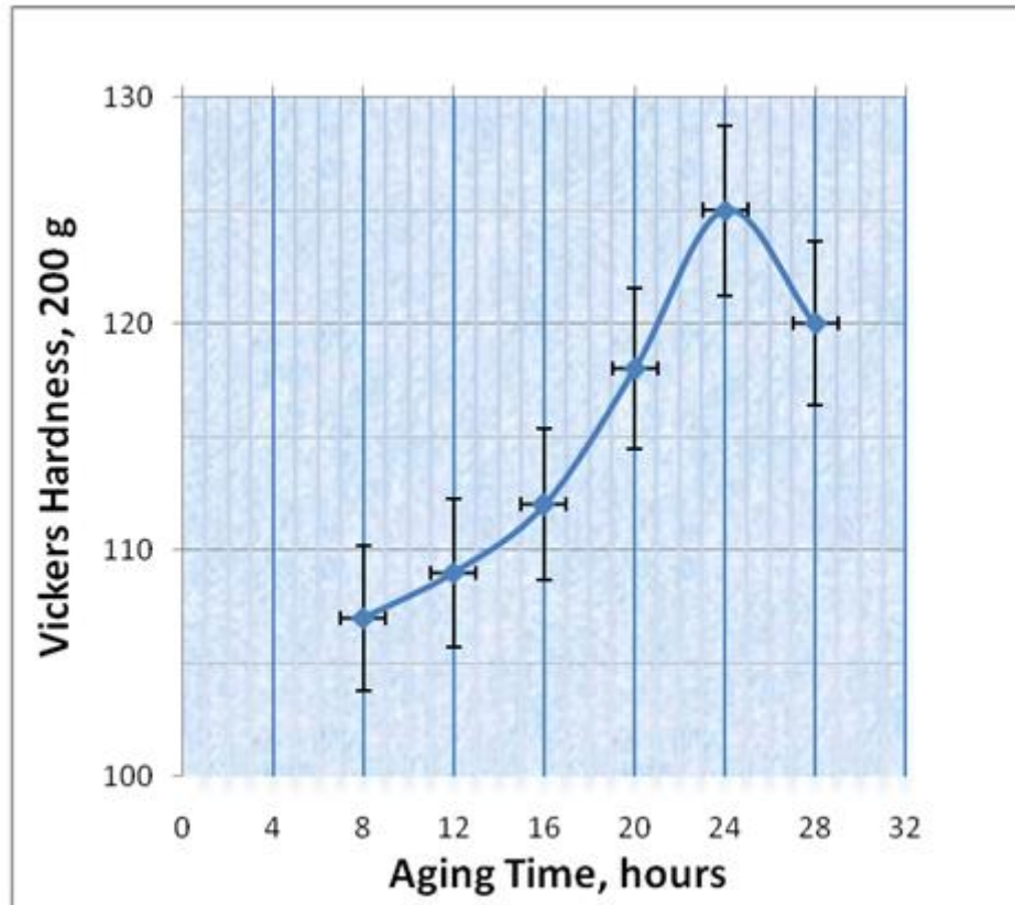
Fig. 2. The hardness values of aged
