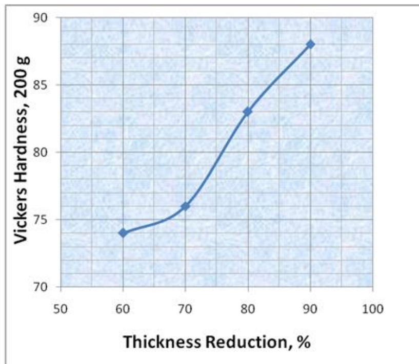
Fig. 1. The hardness values of the homogenized alloys rolled at cryogenic temperature
